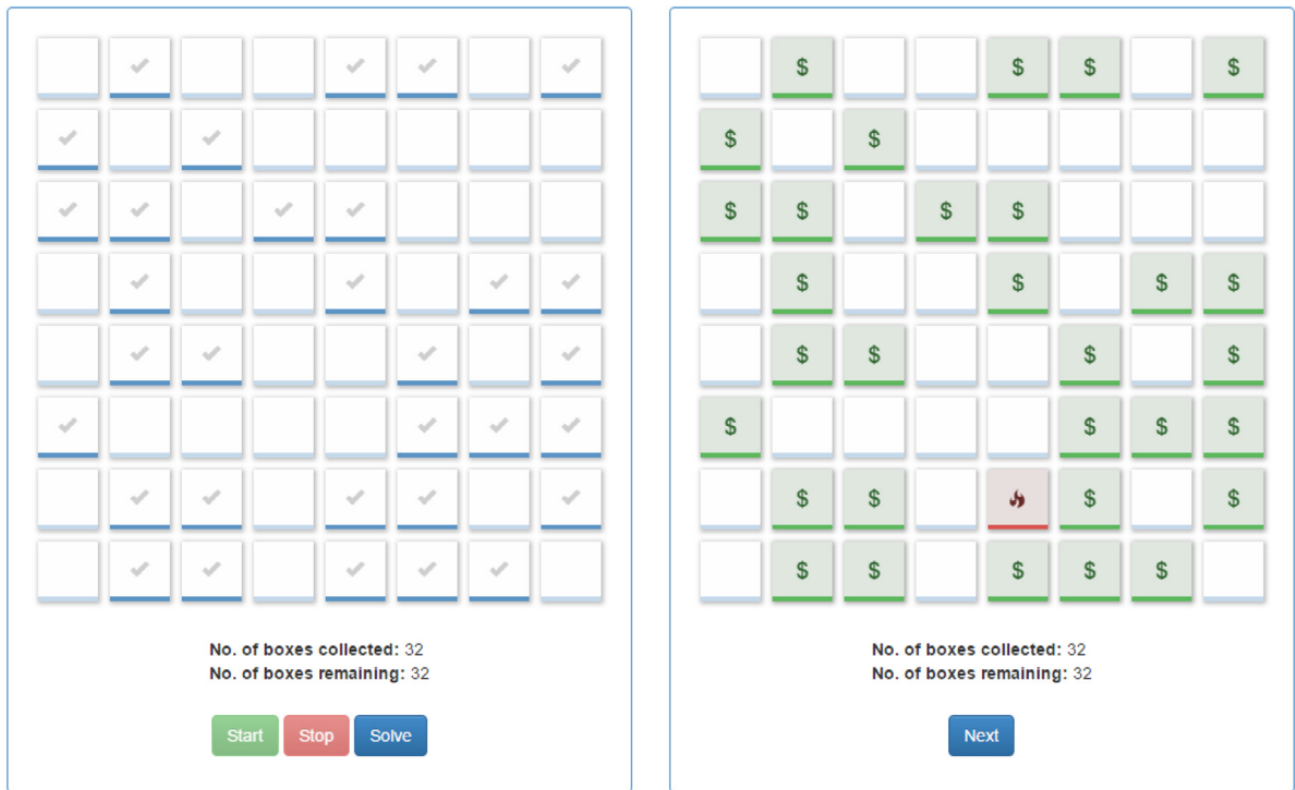
Fig. 1. Bomb risk elicitation task ( \text{num\_rows} = 8, \text{num\_cols} = 8, \text{dynamic} = \text{True}, \text{random} = \text{True}, \text{and feedback} = \text{True} ) after hitting the 'Stop' button (left panel) and after hitting the 'Solve' button (right panel).
